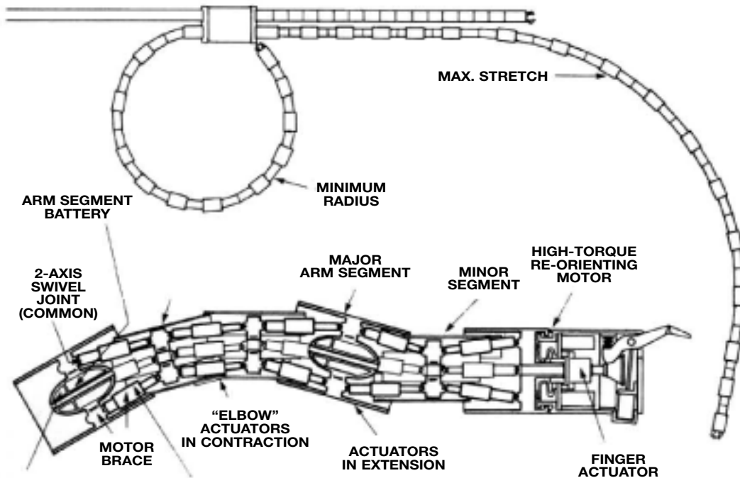
ELECTRONICS PACKAGE MOTOR ARMATURE DRIVES 2 CYLINDERS IN OPPOSITE DIRECTIONS (TYPICAL)
